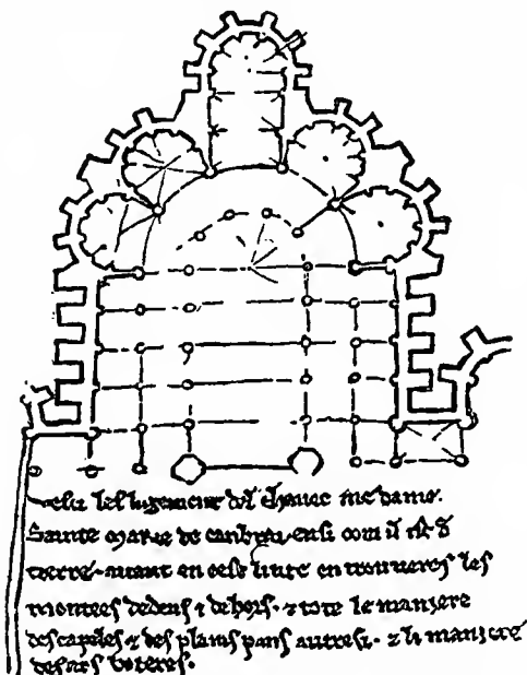
This is a plan of the apse of "Madame Saint Mary"
