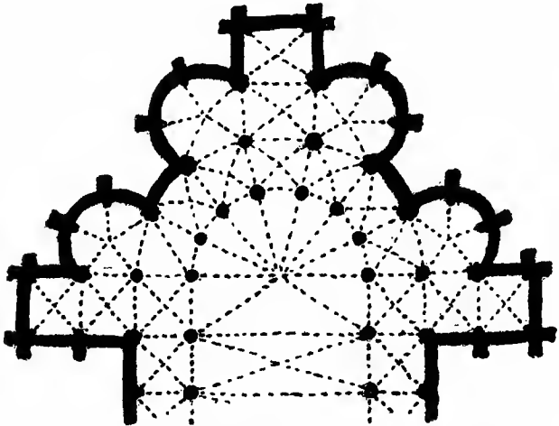
FIG. 72. Destroyed abbey church of Vaucelles, near Cambrai.
