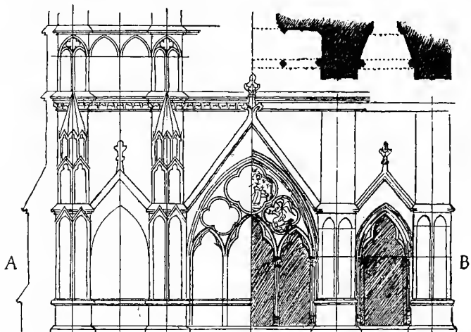
FIG. 116. A, Original design for the west front of a great church of the thirteenth century. B, Suggested interpretation of same.
