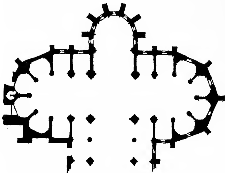
FIG. 63. Plan of church of Cistercian abbey of Chaalis, near Senlis.
