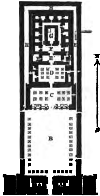
PLAN OF THE TEMPLE OF KDOU. (Built under the Ptolemies B.C. 237-57.)
