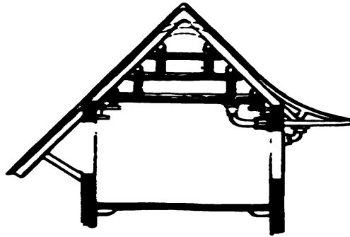
Diagram of Chinese Roof Construction. (From Ferguson.)
