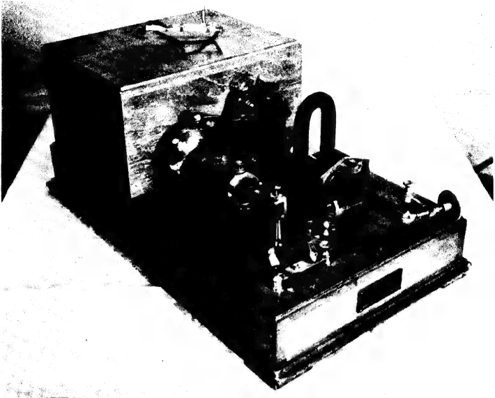
Early receiving equipment which, with the simple coherer as a "heart," first felt the pulse of wireless.
