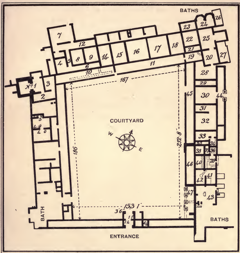
FIG. 11. COURTYARD HOUSE AT NORTHLEIGH, OXFORDSHIRE, AS EXCAVATED IN 1815-16. Room 1, chief mosaic with hypocaust; rooms 8-18, mosaic floors; rooms 21-7 and 38-43, baths, &c.; the west wing had poorer rooms, perhaps for servants. Recent excavations show that this plan represents the house in its third and latest stage; in the corridor (10) a part of the earlier house-front is shown by dotted lines. The pottery found in the recent excavations suggests that the first house on this spot was built not later than the early second century.
