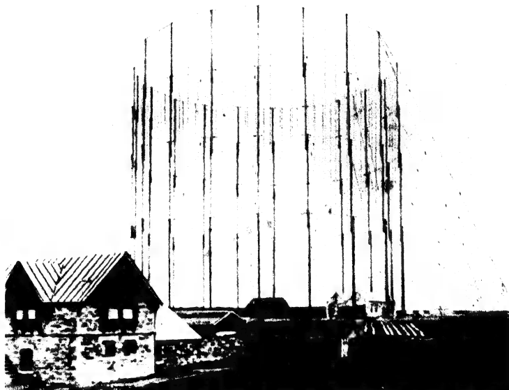
Poldhu's first circular aerial on the southwest tip of England, the site from which the pioneer transoceanic signal took wing for a flight to Newfoundland where Marconi plucked it from space.
